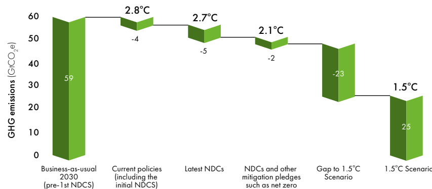
Contribution of NDCs and other pledges to limiting global warming, as of November 2021
